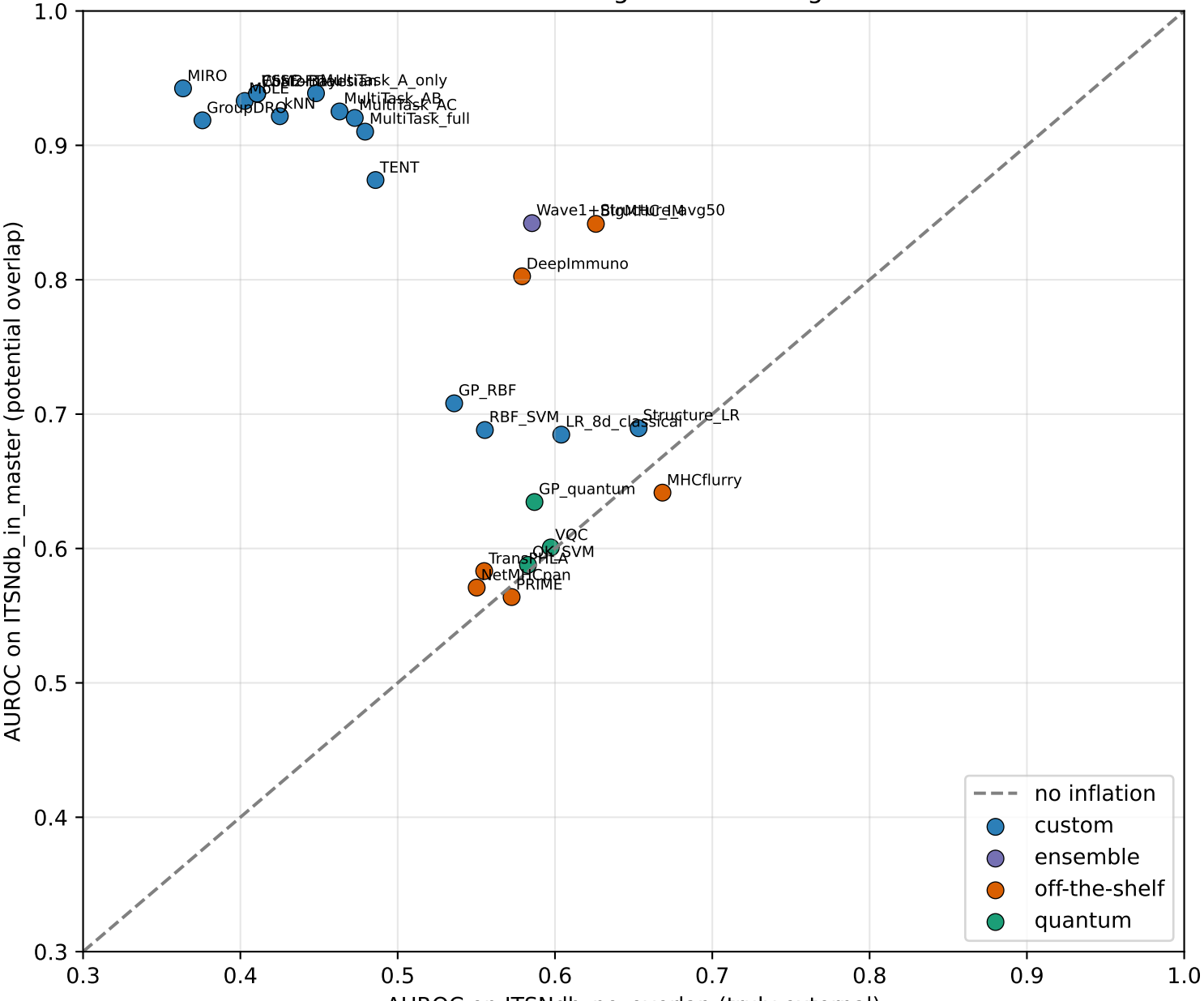
Wave 10 — leakage inflation diagonal
