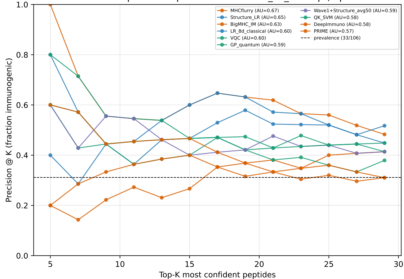
Wave 10 — selective prediction precision on ITSNdb_no_overlap (top 10 methods)
