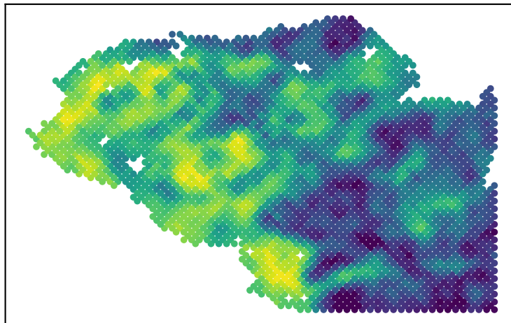
P2 observed
