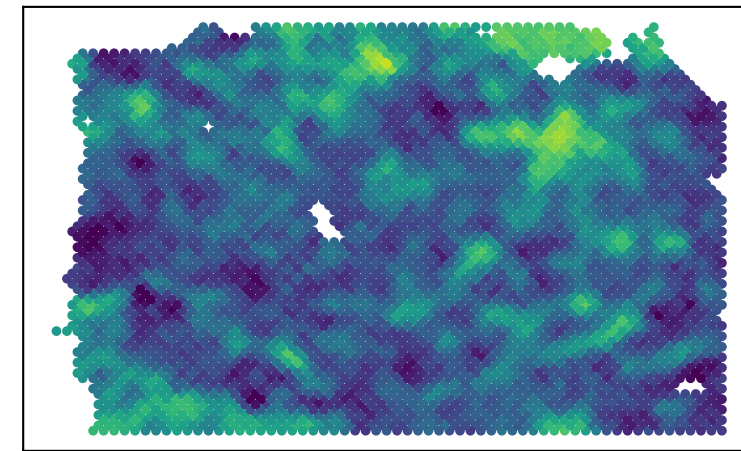
P4 observed
