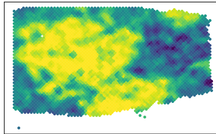
P3 observed
