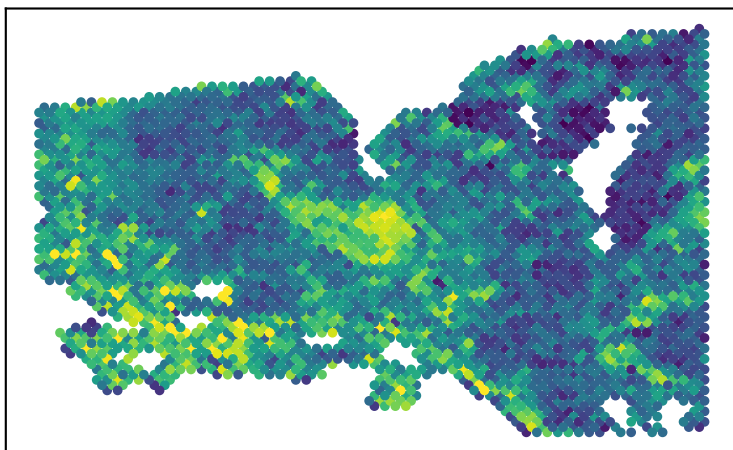
P1 H&E-predicted
