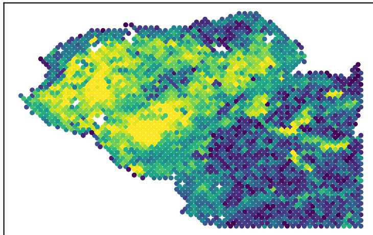
P2 H&E-predicted
