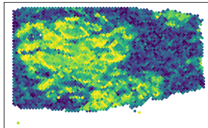
P3 H&E-predicted
