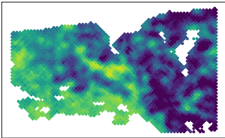
P1 observed
