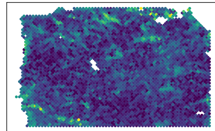
P4 H&E-predicted
