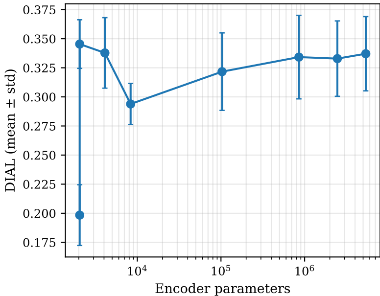
Figure 4 — Foundation-model scaling: NEGATIVE result (slope r^2 = 0.19 , near zero) DIAL vs encoder size — no monotonic decrease Target AUC vs encoder size — also no monotone trend
