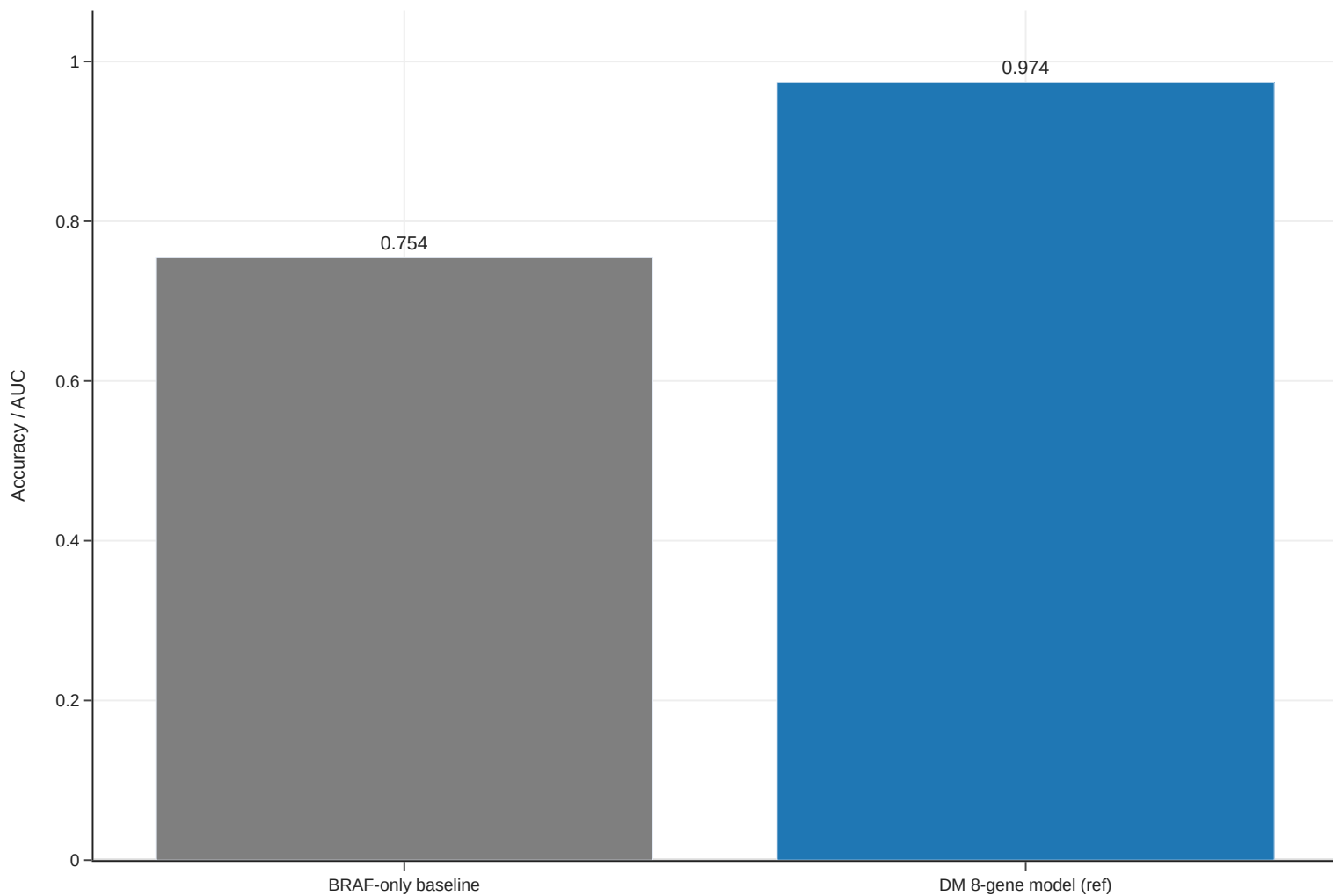
SuppFig10 — BRAF-only baseline vs 8-gene DM model
