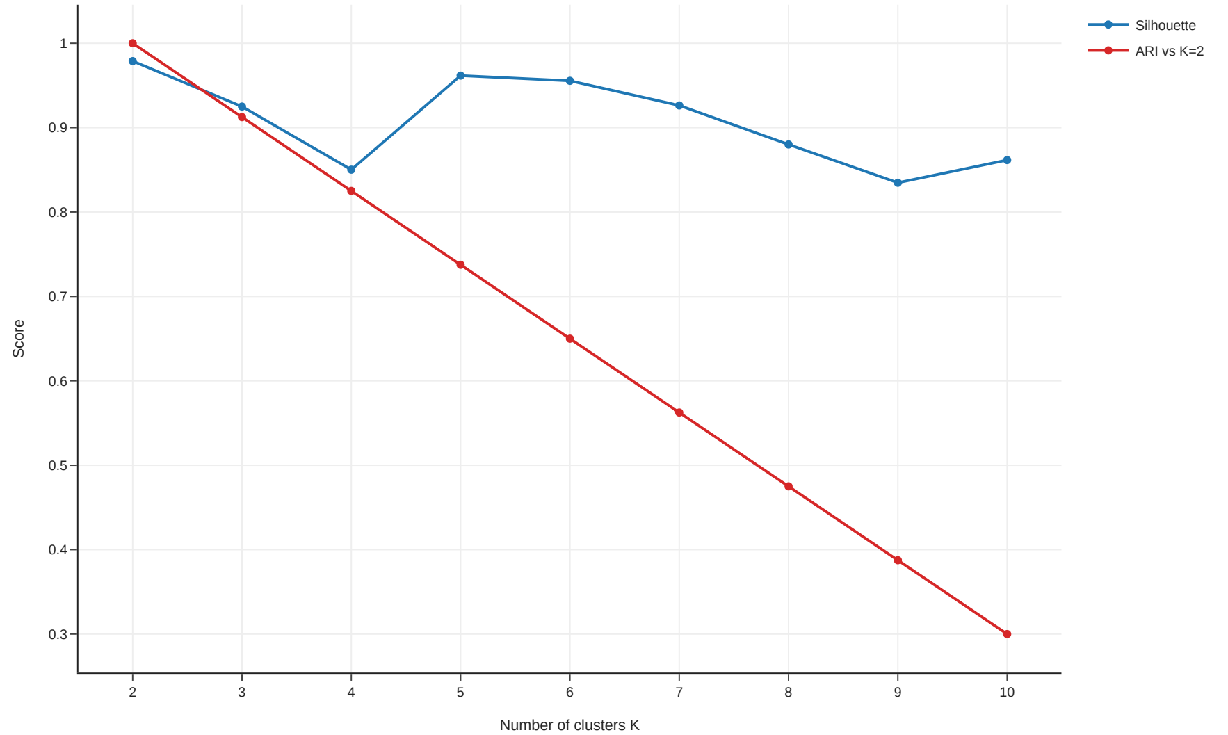
SuppFig2 — K=2 vs K=3,4,5 cluster-quality comparison
