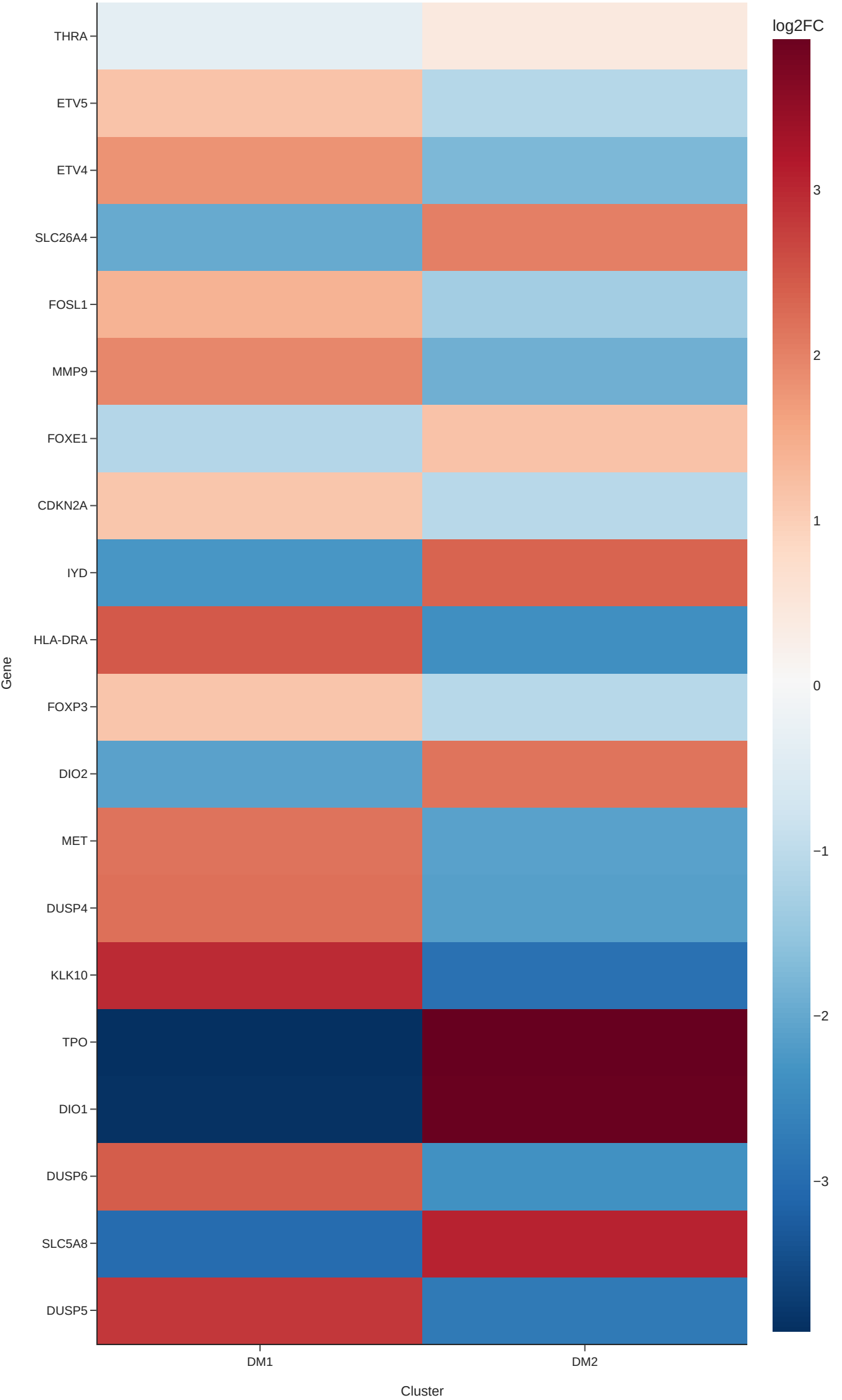
SuppFig6 — Full marker heatmap (n=20 cluster-defining genes, FDR<1e-30)
