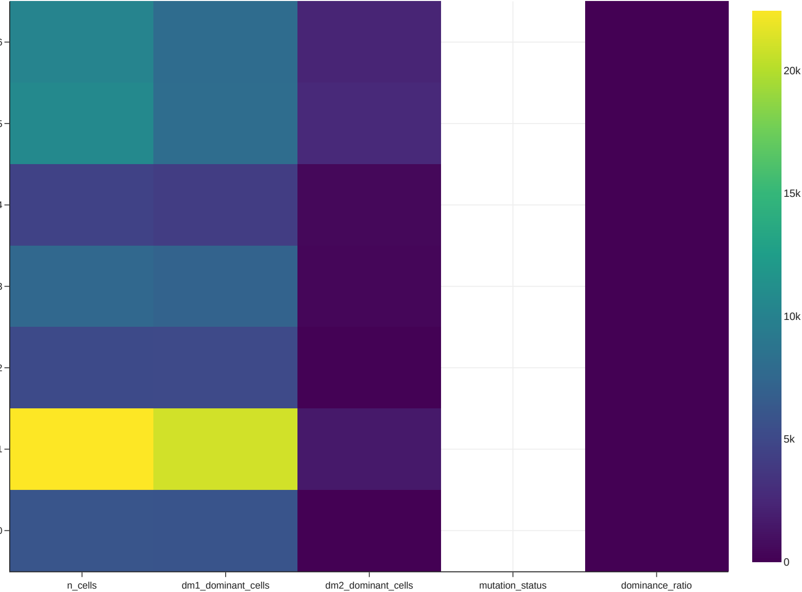
SuppFig7 — scRNA per-patient DM landscape (numeric features)
