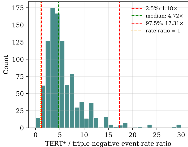
Figure 8E.ii — Effect-size CI (median 4.7\times , 95 % CI 1.2\times - 17.3\times )
