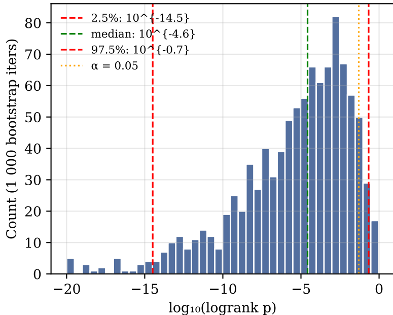
Figure 8E.i — Bootstrap p distribution (median p = 2.6 \times 10^{-5} ; 93 % iter p < 0.05 )
