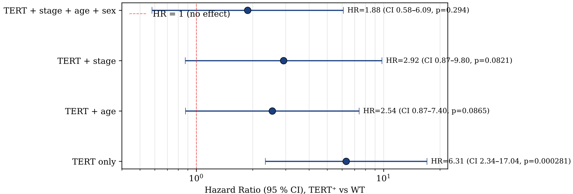
Figure 8B — Forest plot of TERT + Hazard Ratio (lifelines penalizer = 0.01) Univariate signal collapses to non-significant after stage + age adjustment
