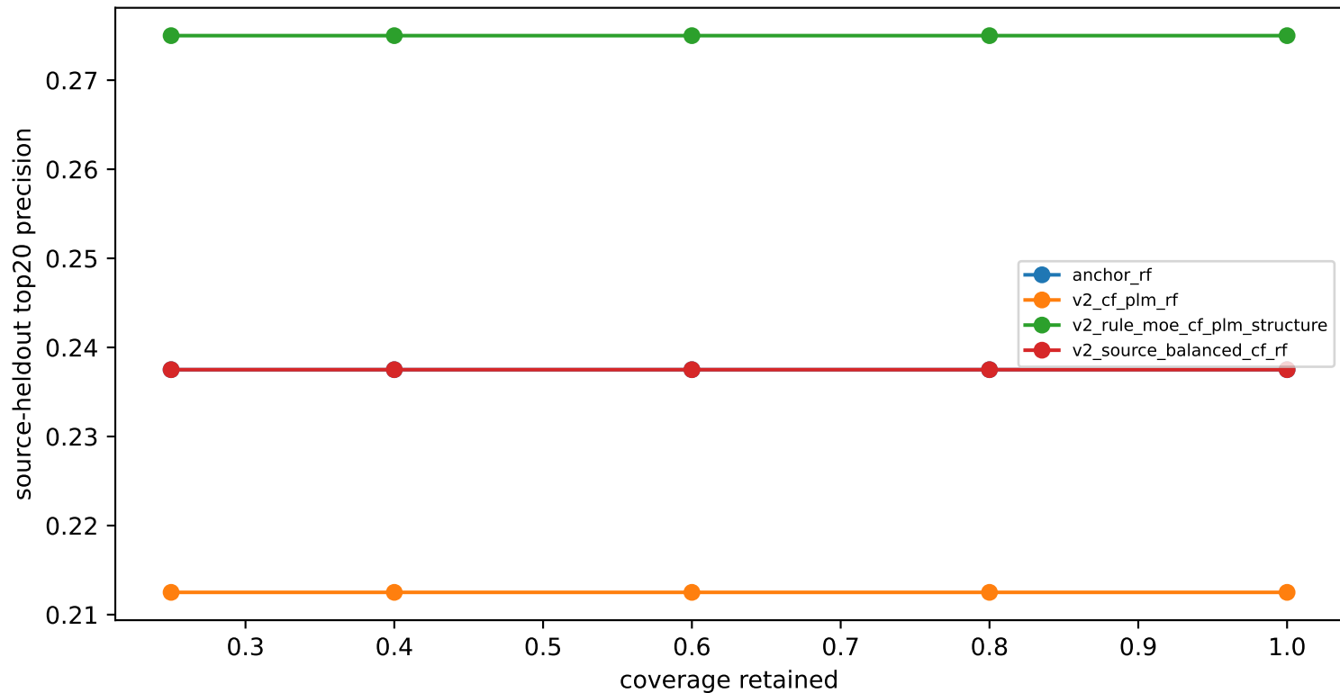
Source-heldout internal abstention curve
