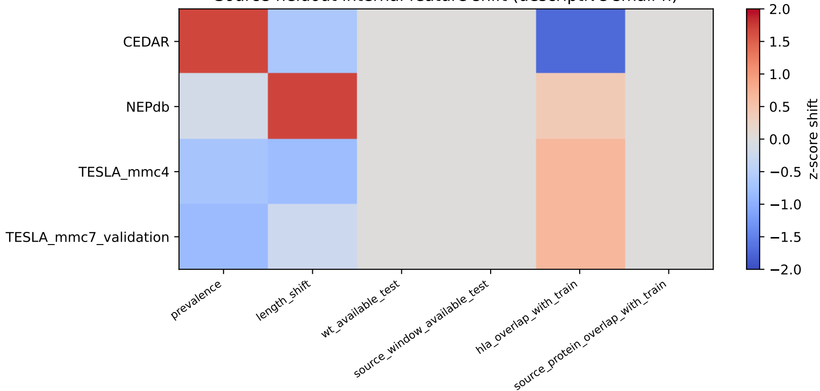
Source-heldout internal feature shift (descriptive small-n)
