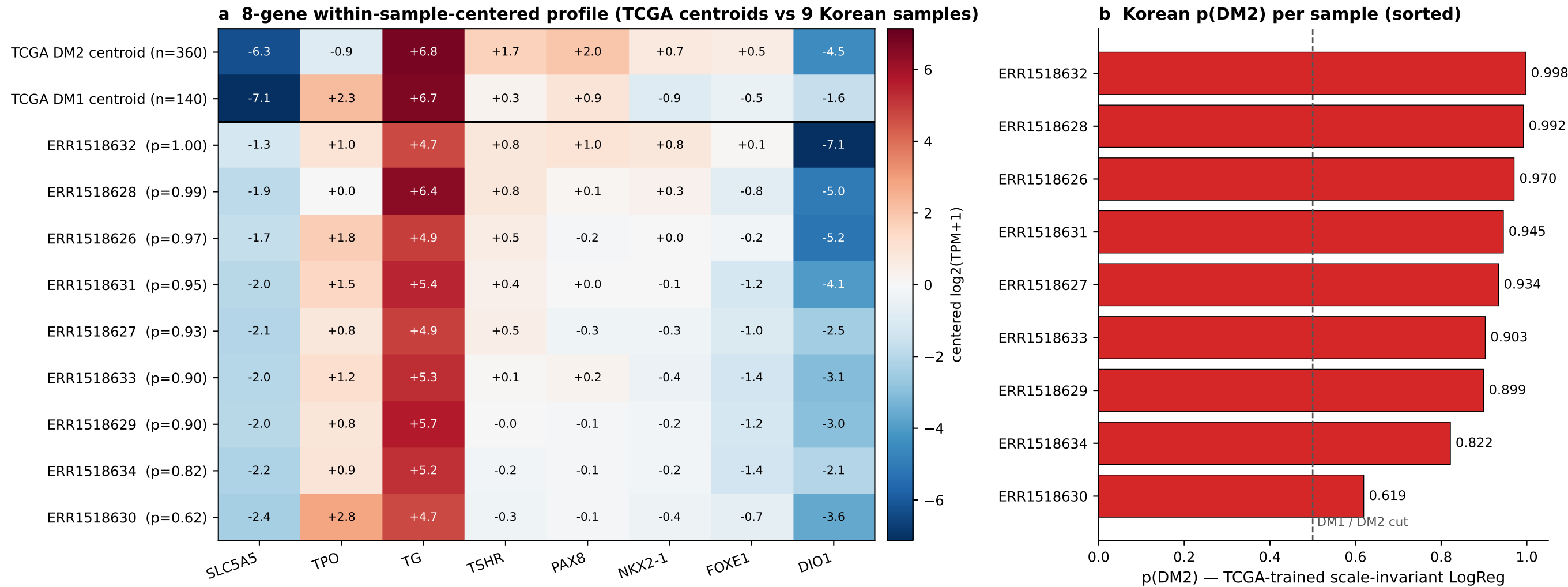
Fig K2. PRJEB11591 Korean PTC pilot (n = 9) — within-sample-centered 8-gene profile vs TCGA DM1/DM2 centroids; 9/9 → DM2 (mean p = 0.898)
