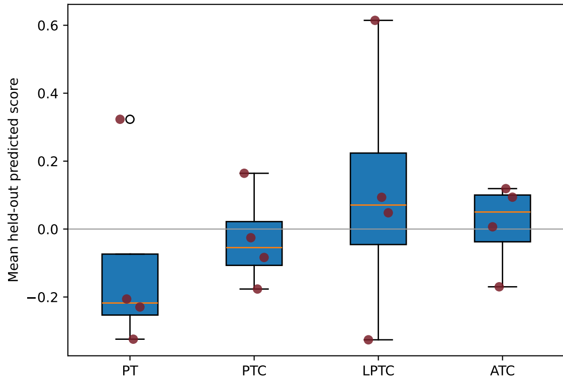
Slide mean morphology-DM1 score by spatial stage
