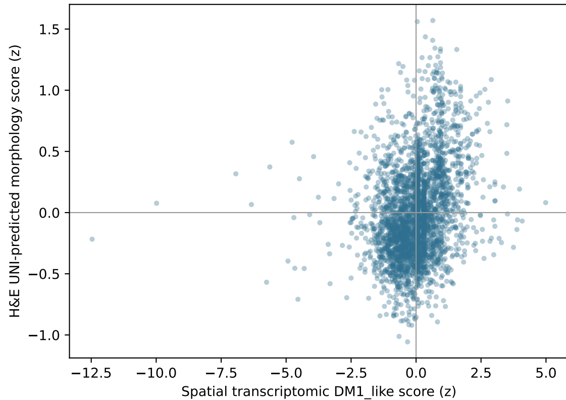
Leave-slide-out spots: \rho=0.30 , p=6.7\text{e-}68
