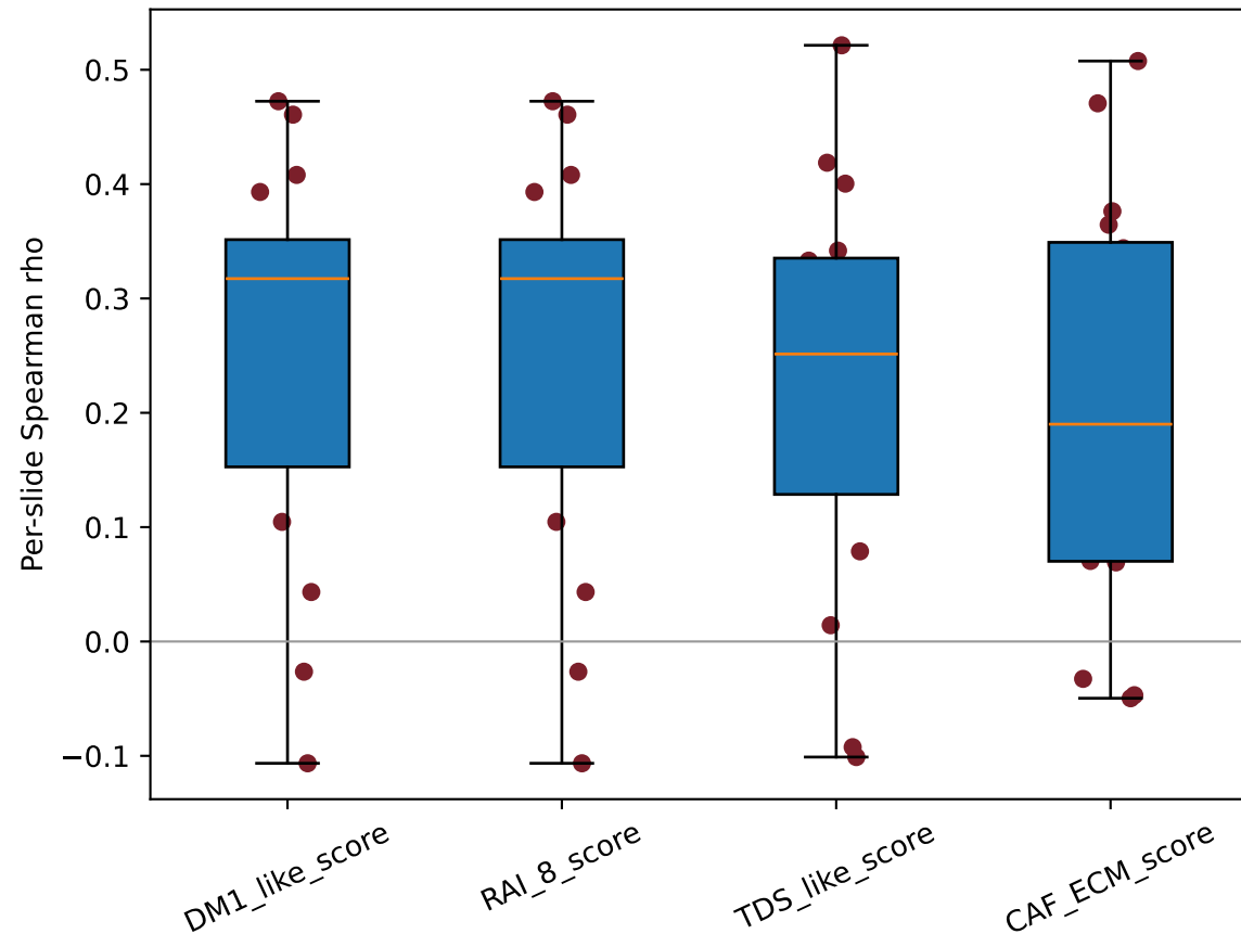
Slide-level robustness for top programs
