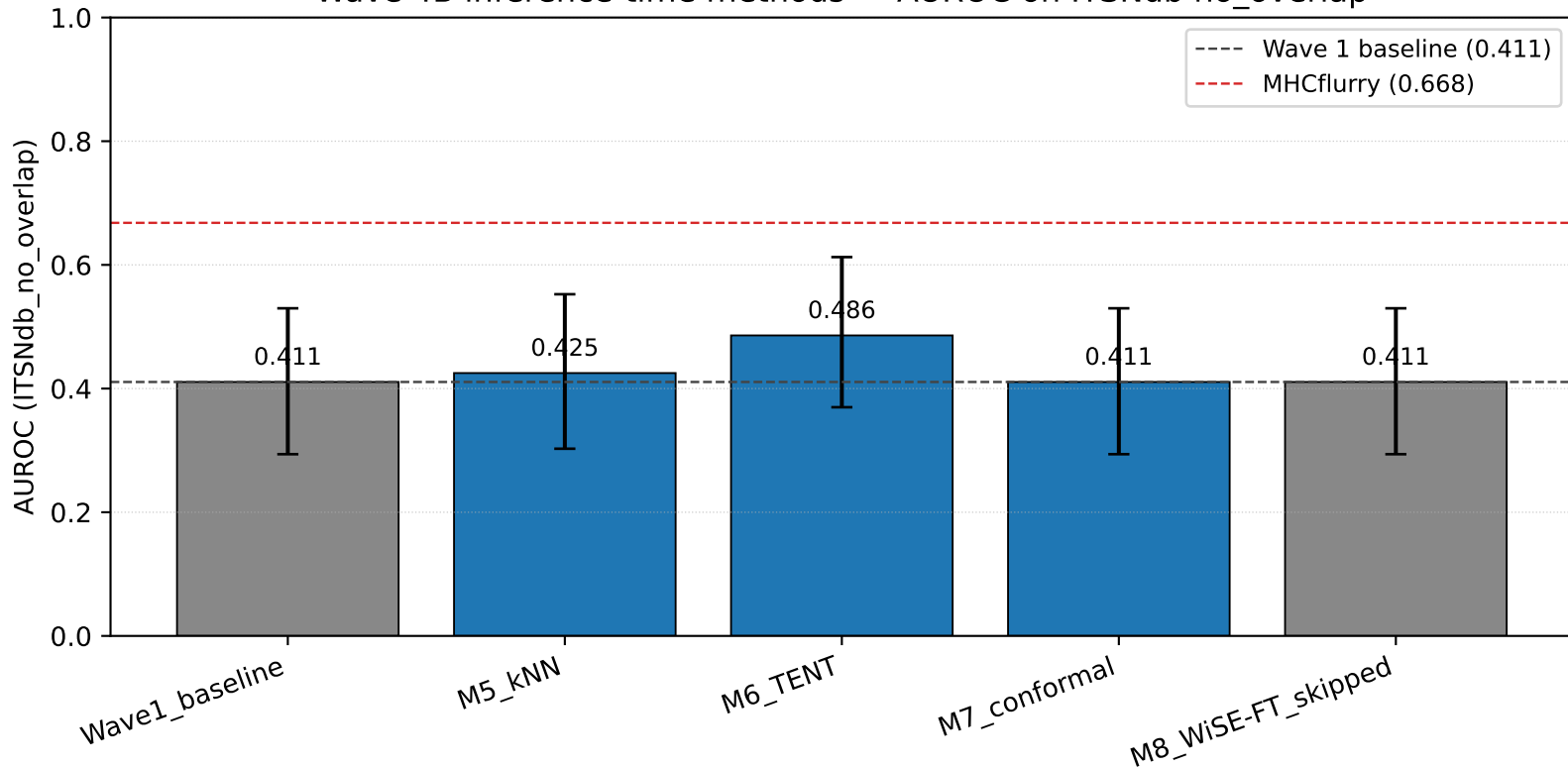
Wave 4B inference-time methods — AUROC on ITSNdb no_overlap
