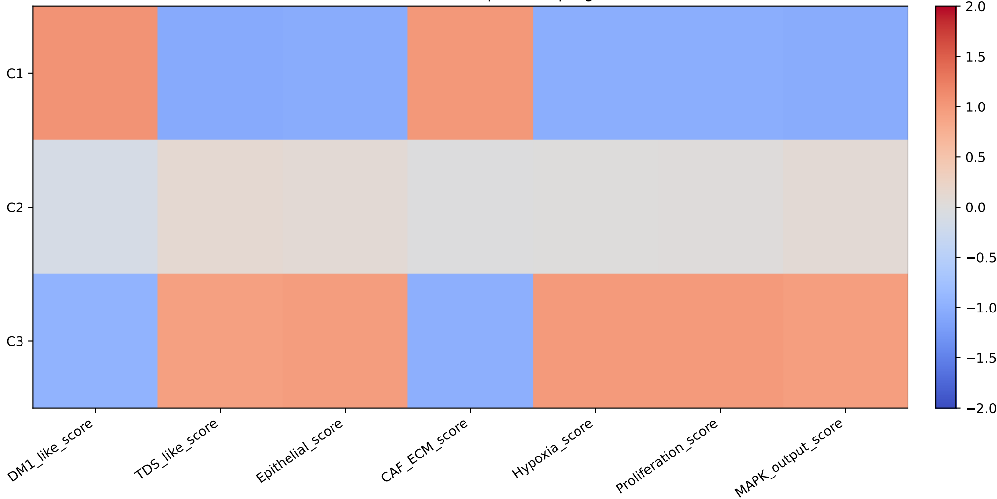
Predicted ST cluster expression programs
