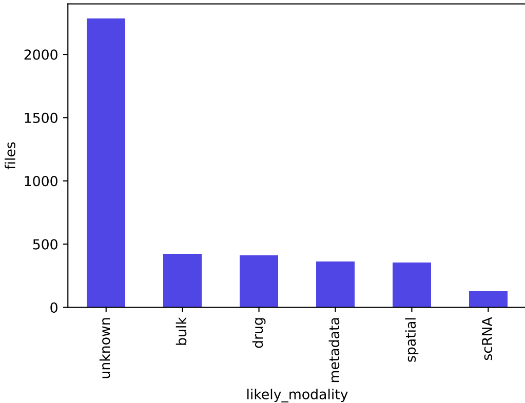
Data coverage
