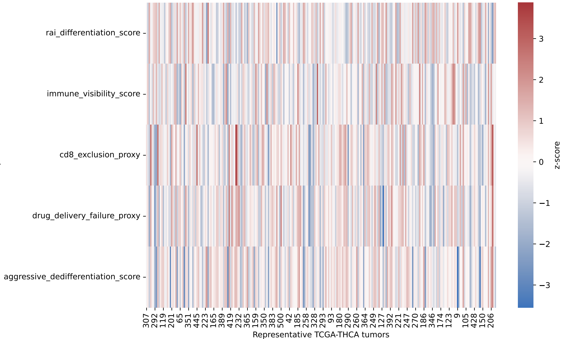
Figure 2. TCGA Therapeutic Vulnerability Landscape
