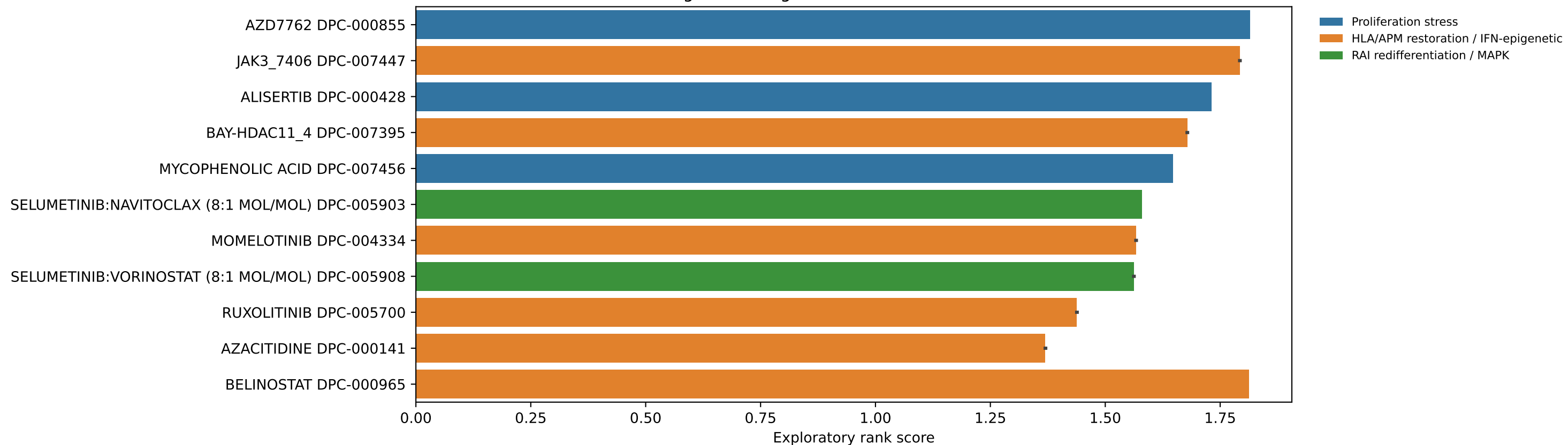
Figure 6. Drug/Perturbation Candidate Pilot
