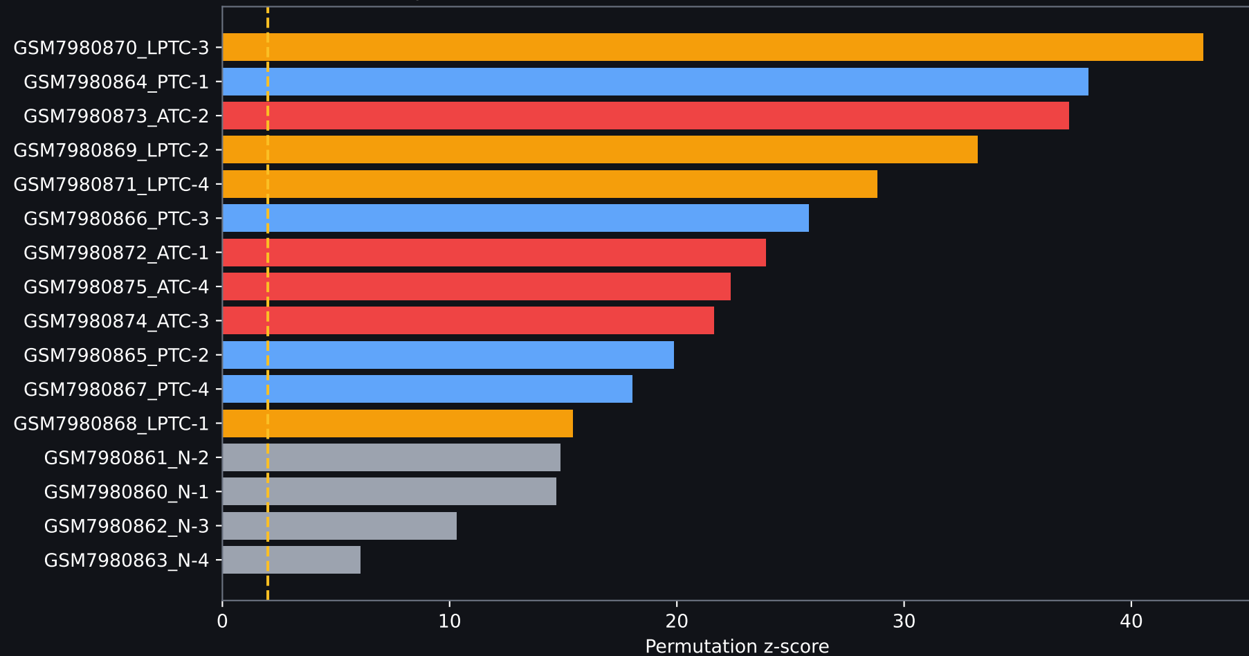
Spatial same-niche KNN coherence across GSE250521 slides
