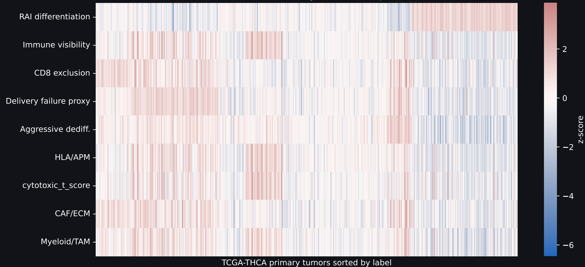
TCGA vulnerability axes heatmap
