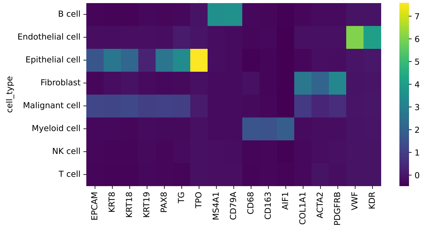
scRNA marker expression by annotated cell type
