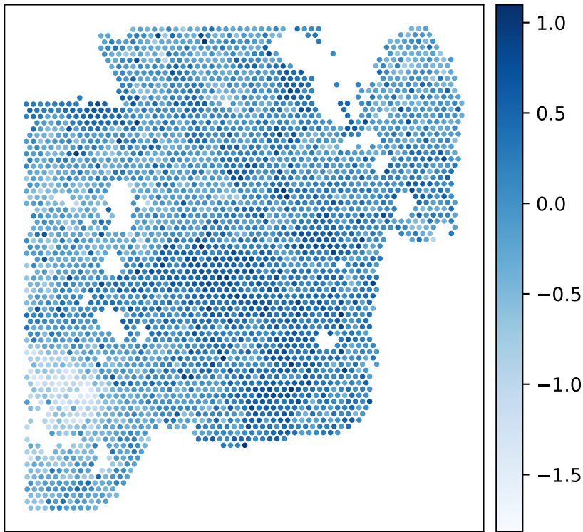
GSM7980860_N-1 RAI differentiation
