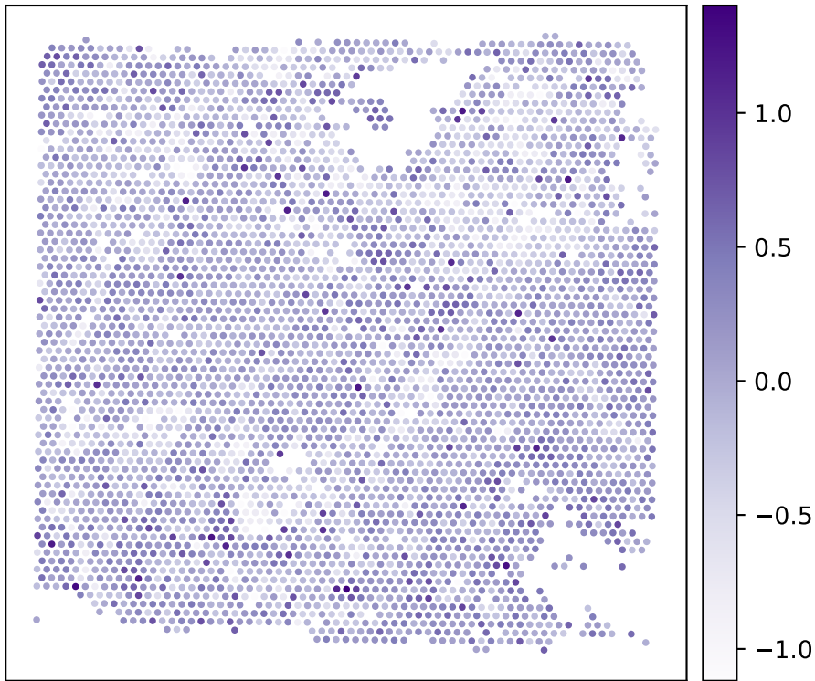
GSM7980869_LPTC-2 HLA/APM
