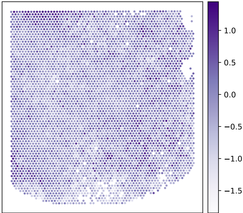
GSM7980872_ATC-1 HLA/APM
