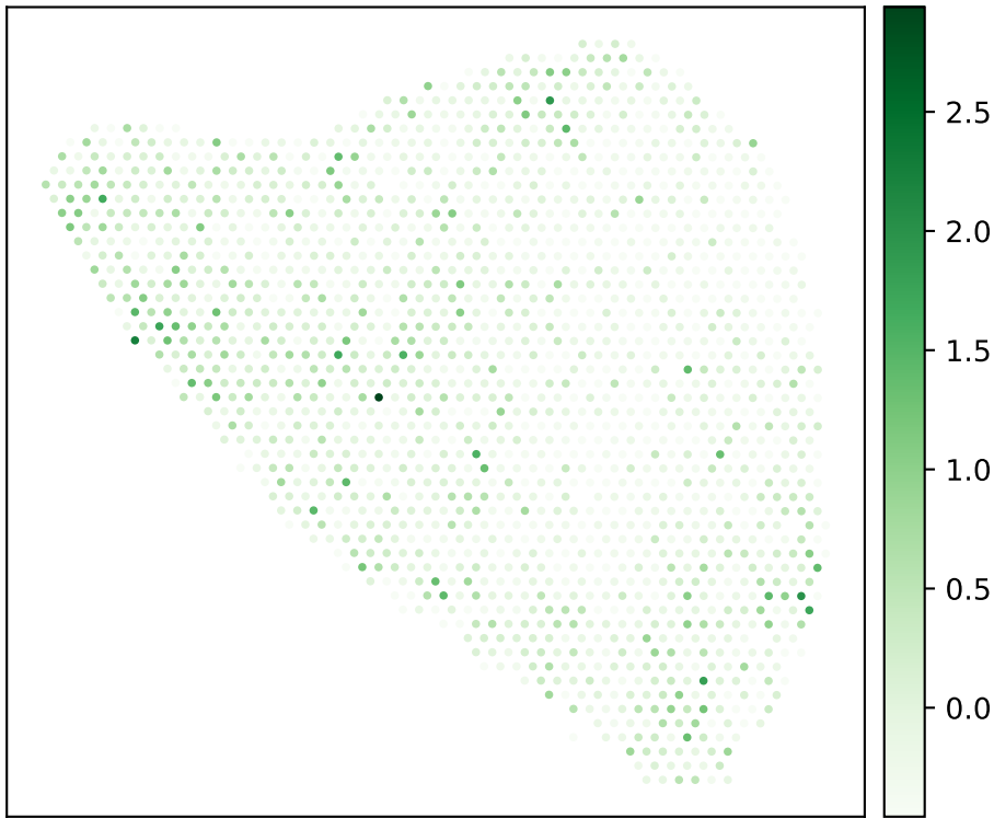
GSM7980874_ATC-3 CD8/cytotoxic
