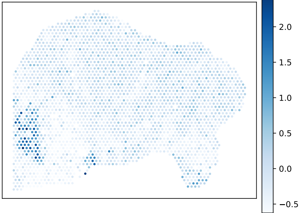
GSM7980875_ATC-4 RAI differentiation
