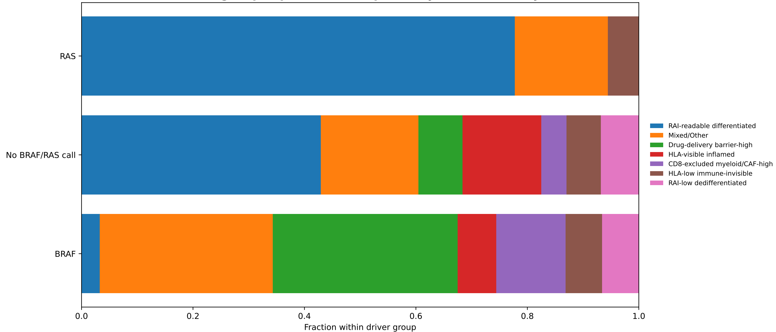
TCGA driver groups split into multiple K-Thyro vulnerability labels
