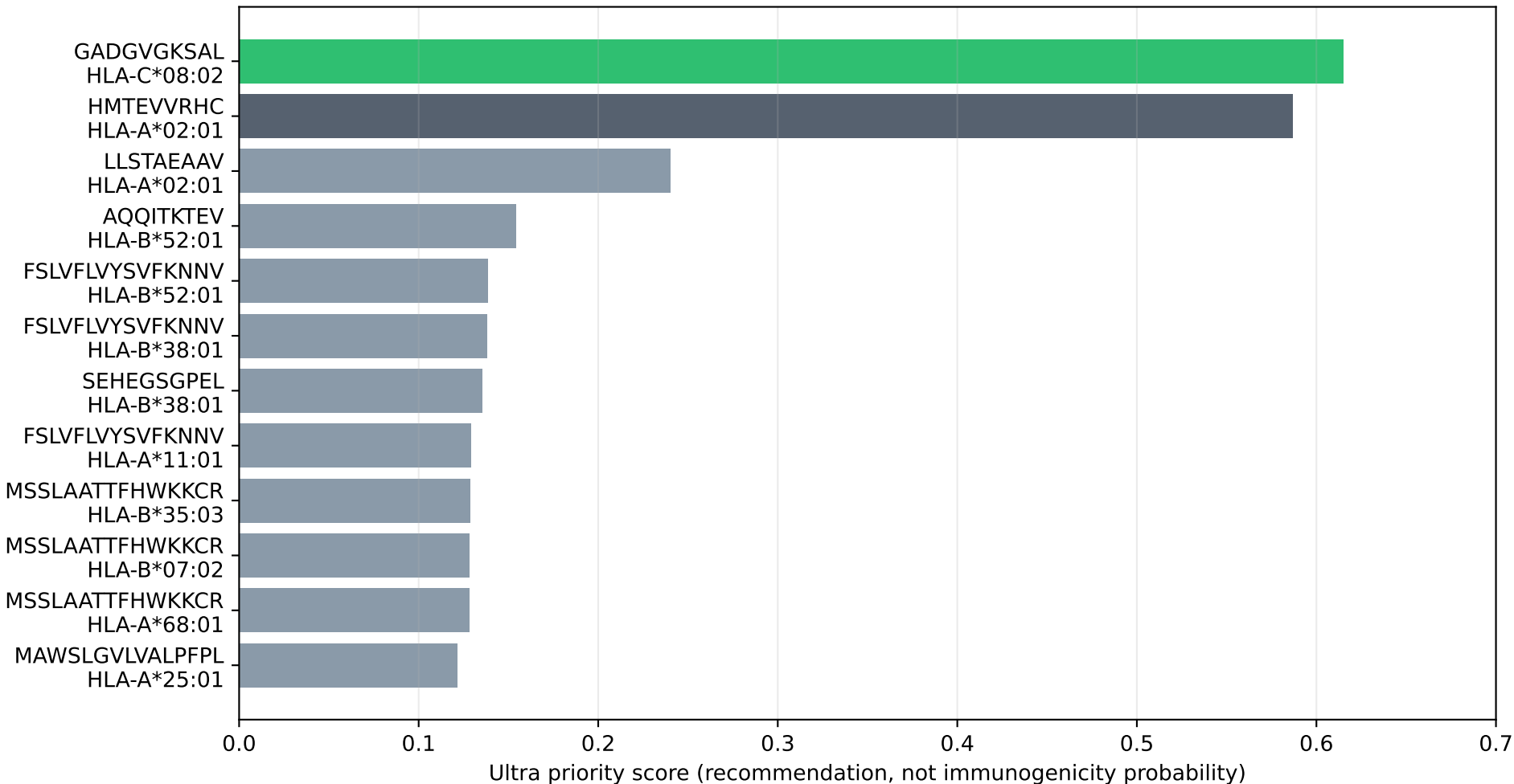
CROSS-Neo-TCR-MD wetlab prioritization
