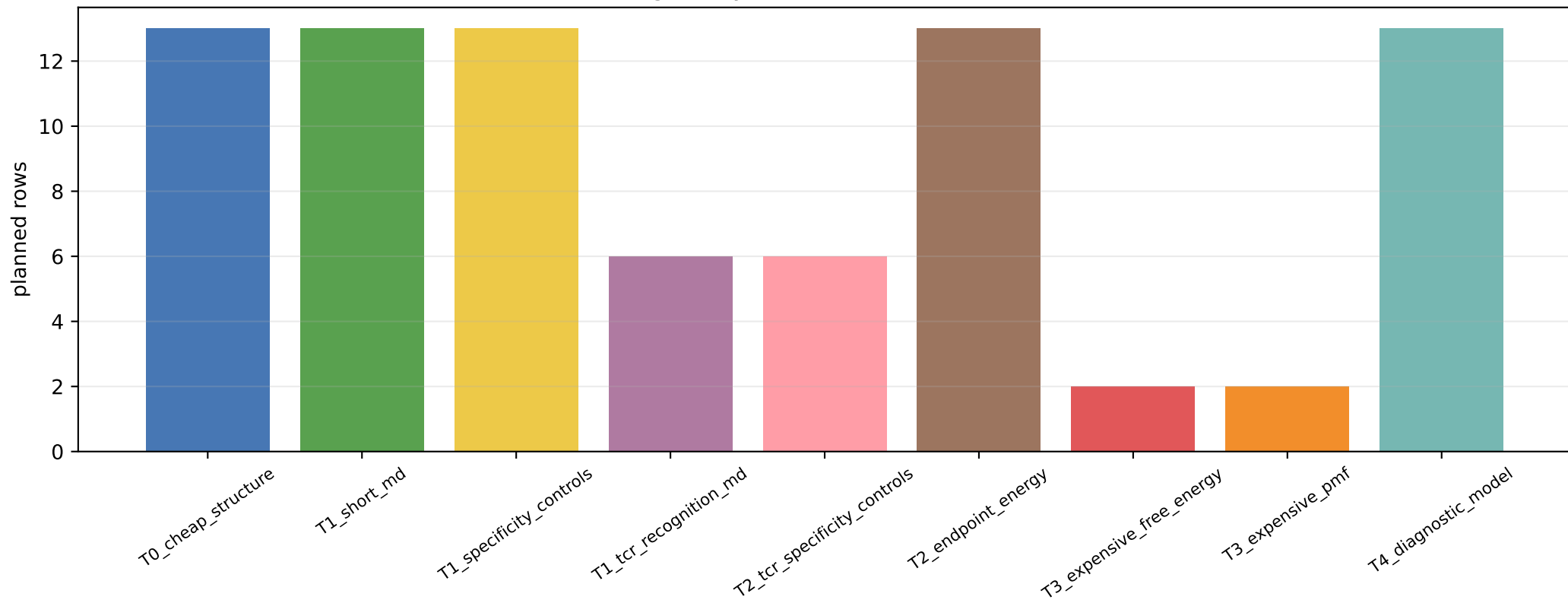
Immunogenicity simulation escalation ladder
