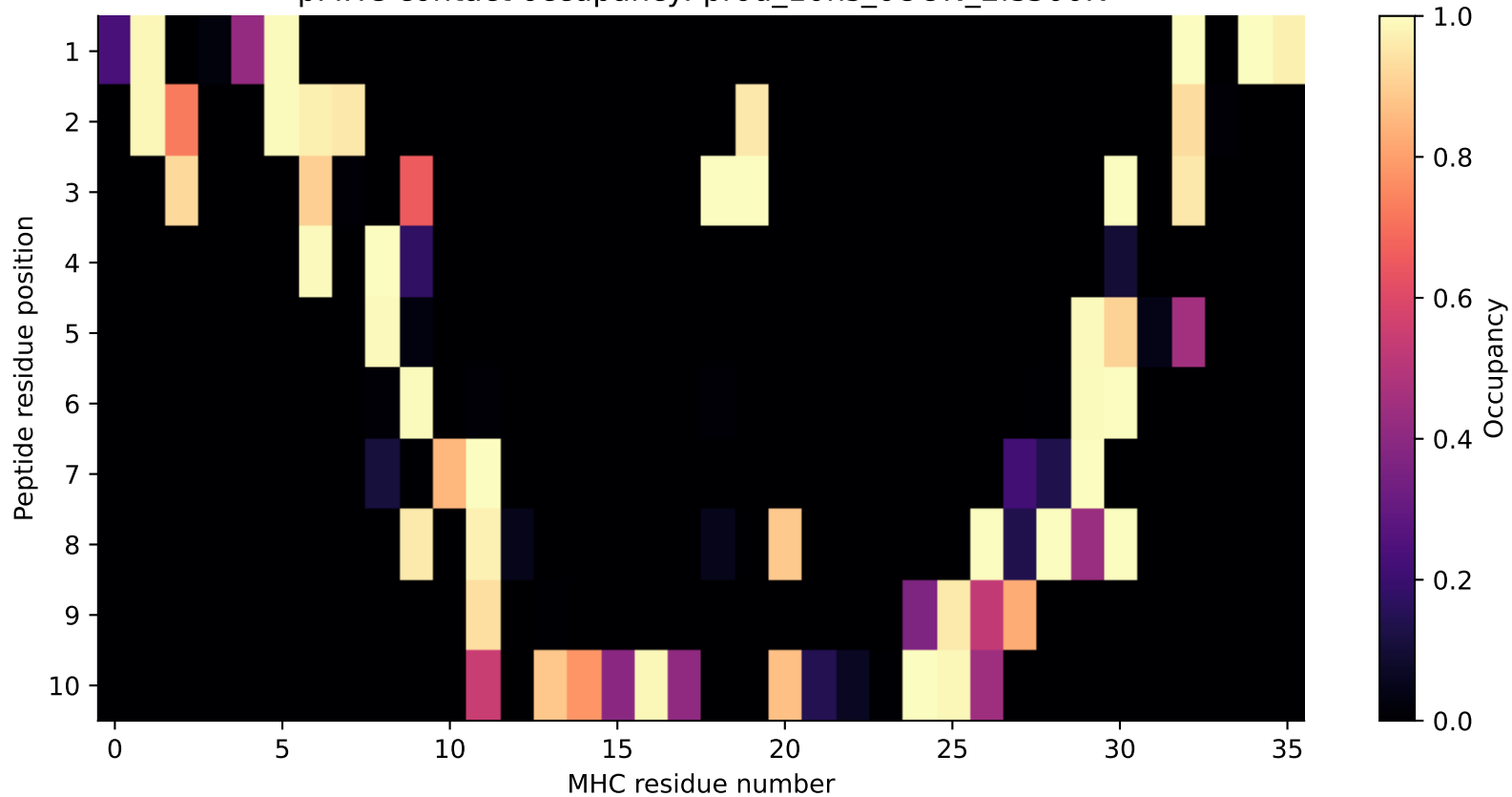
pMHC contact occupancy: prod_10ns_6UON_2fs300K
