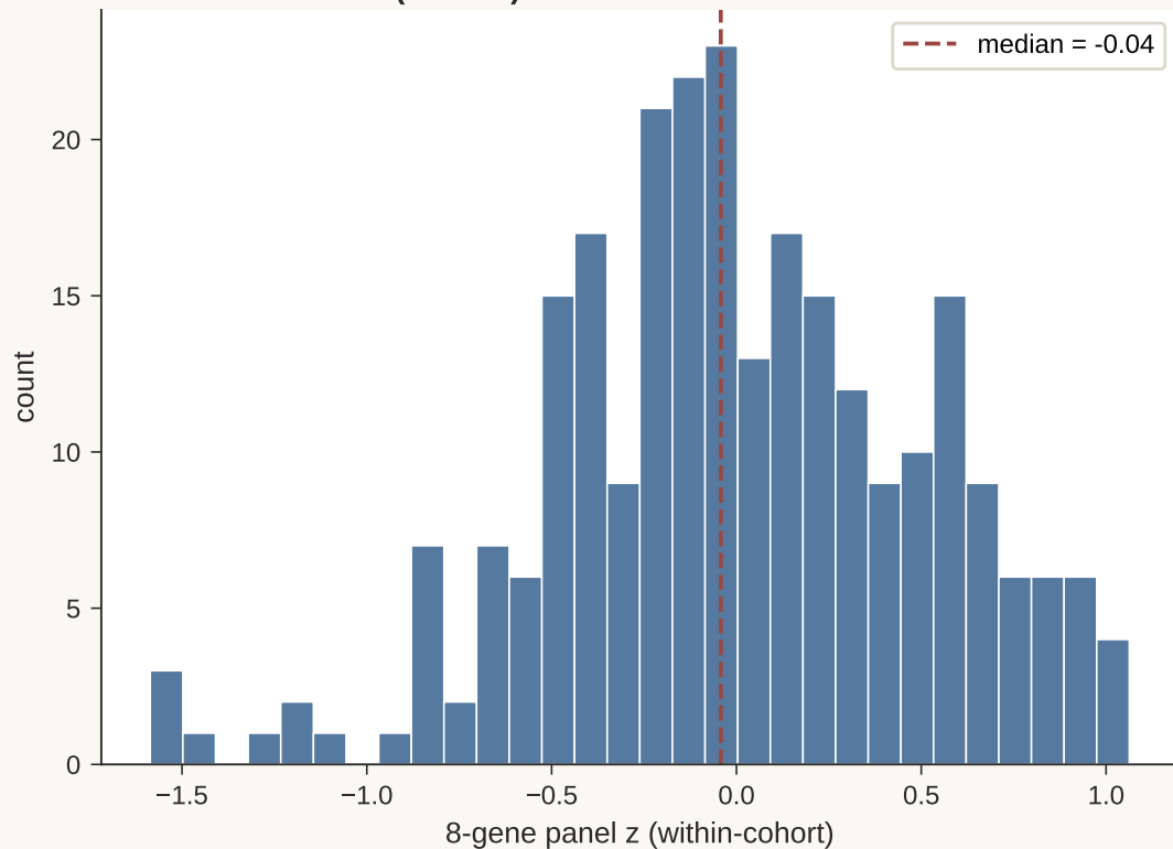
Panel z distribution (n = 260)
