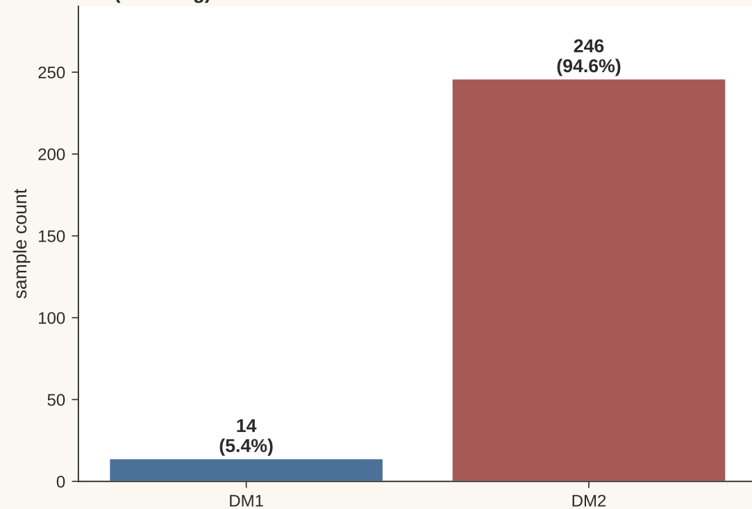
DM (silencing) call distribution
