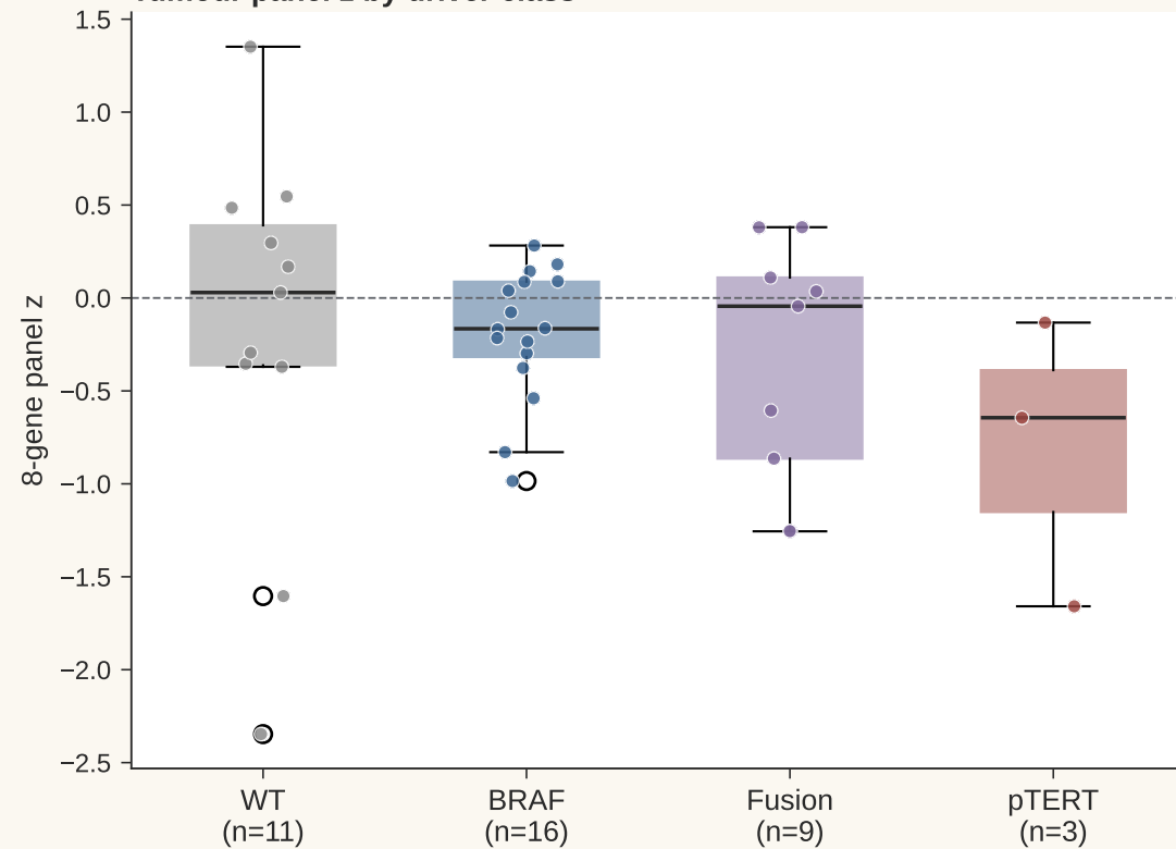
a Tumour panel z by driver class
