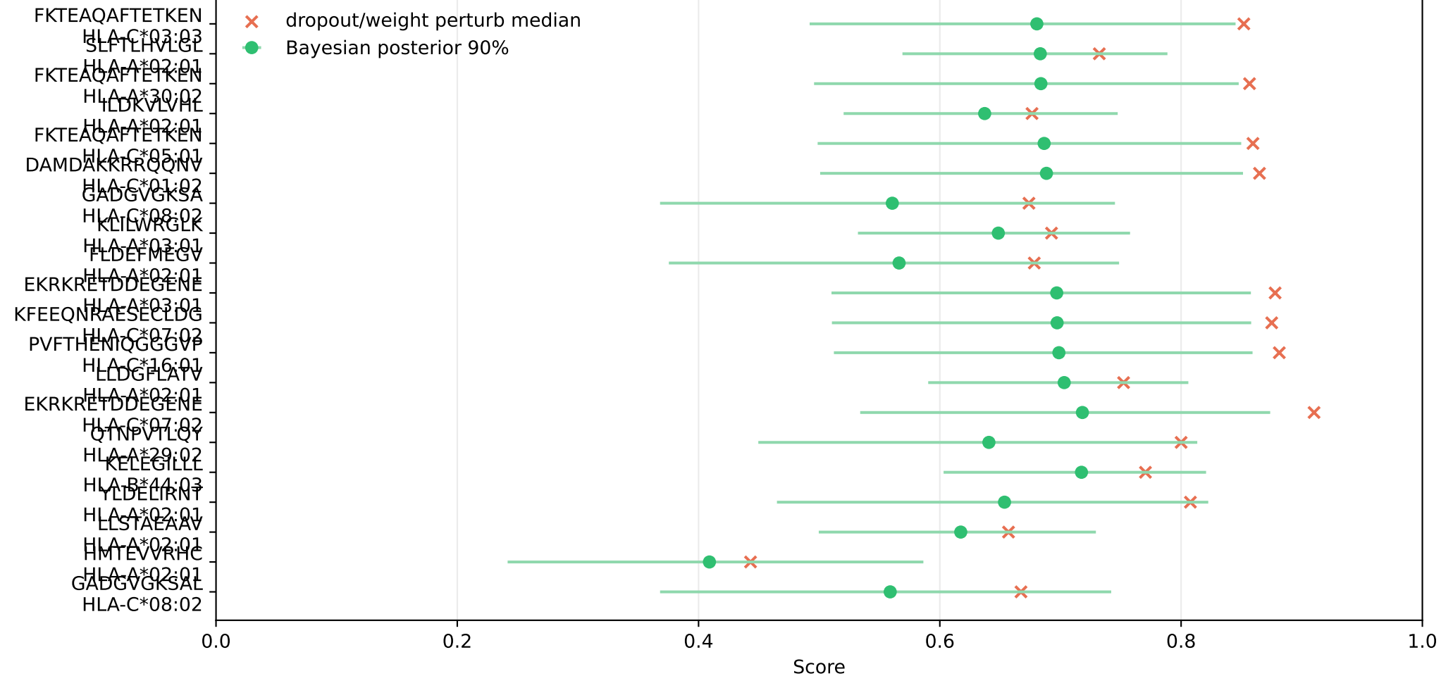
Bayesian and dropout uncertainty for highest-action candidates
