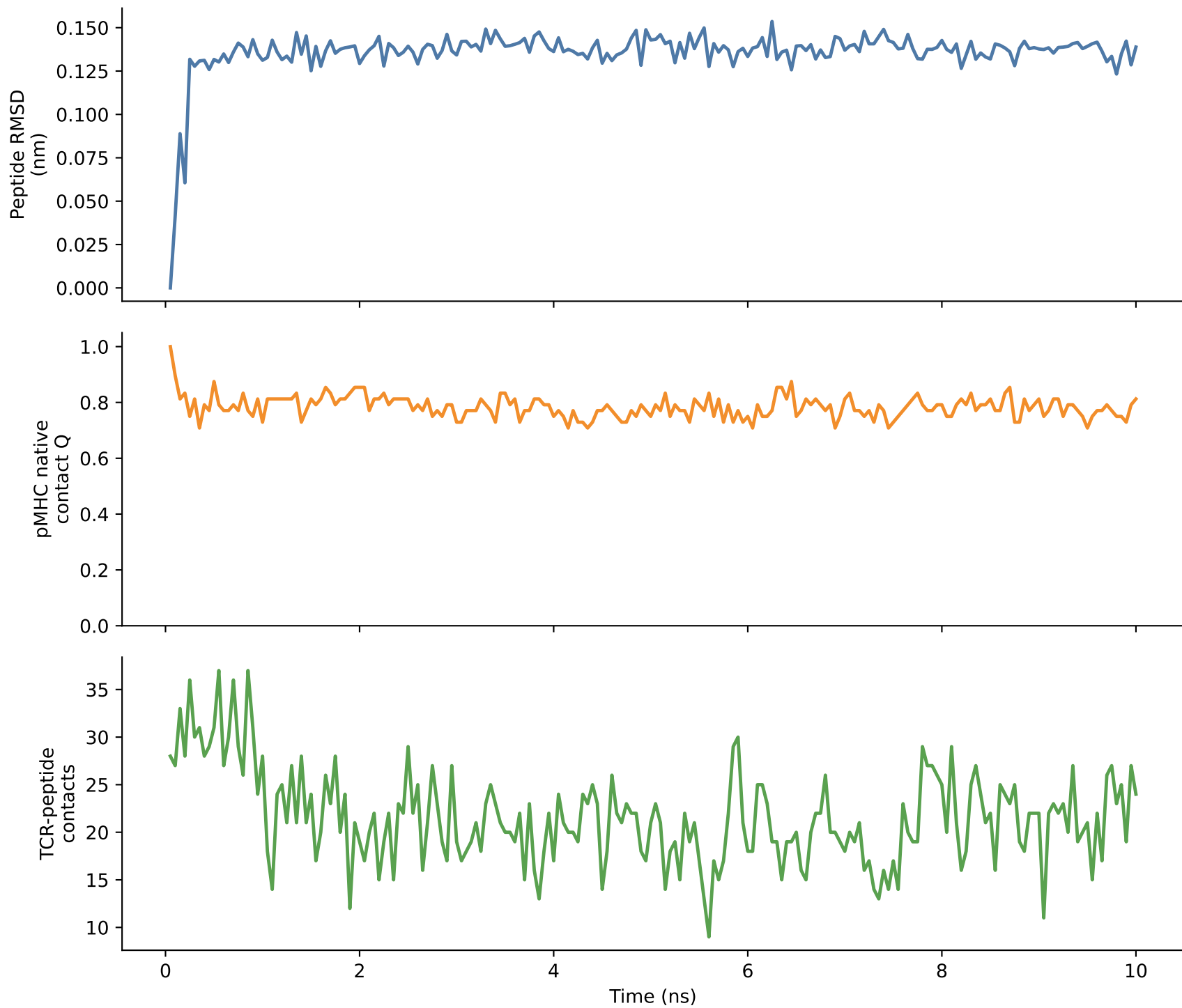
GADGVGKSAL / HLA-C*08:02 / 6UON 10 ns structural audit
