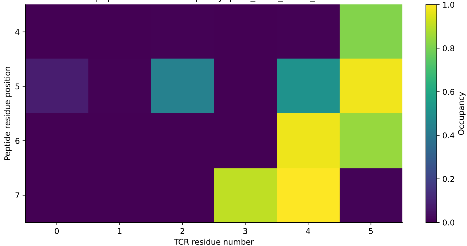
TCR-peptide contact occupancy: prod_10ns_6UON_2fs300K
