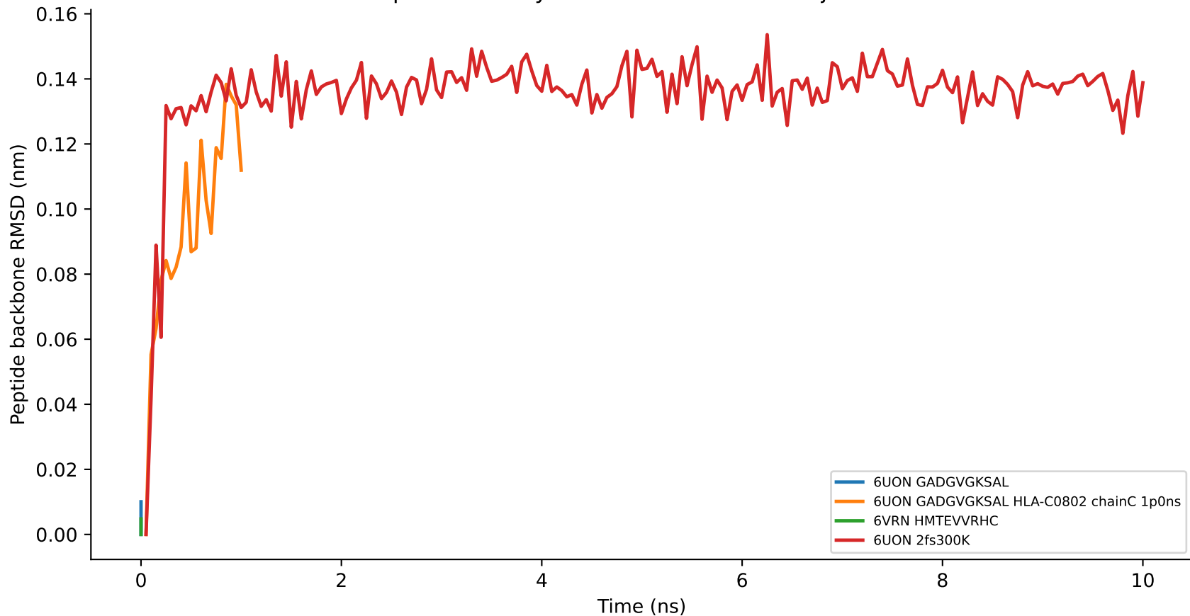
Peptide stability across available MD trajectories
