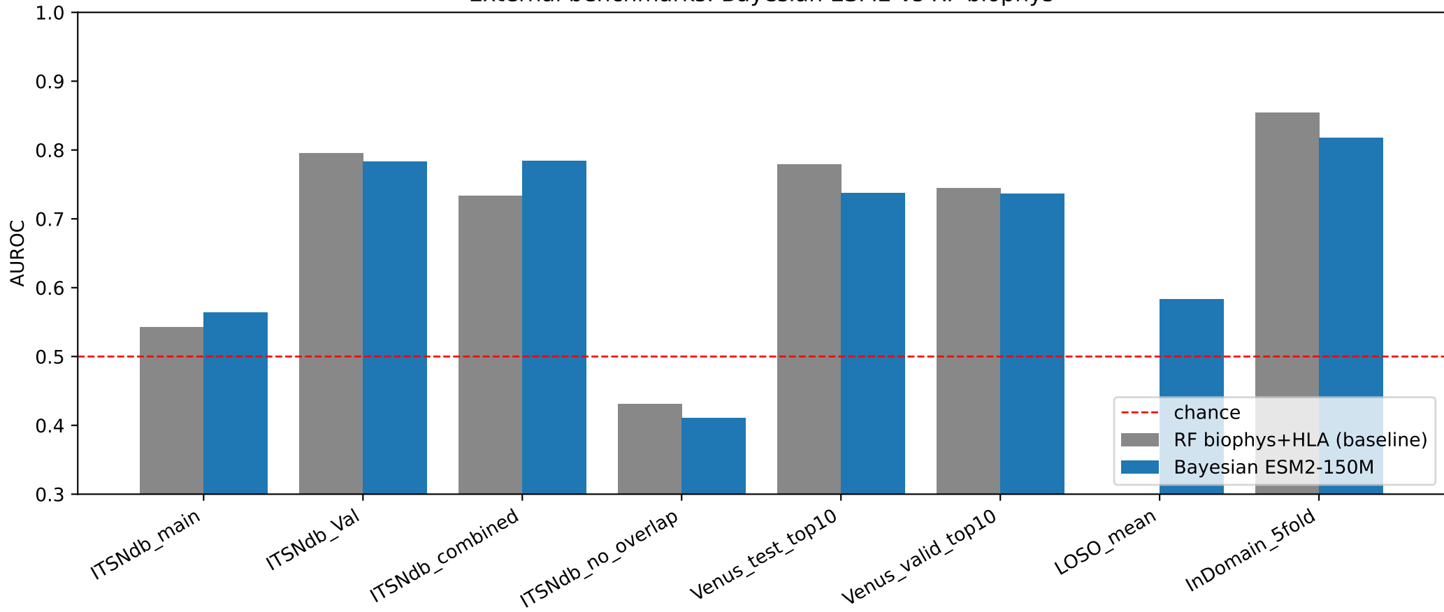
External benchmarks: Bayesian ESM2 vs RF biophys
