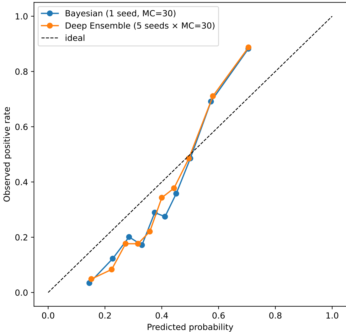
Calibration — in-domain 5-fold (ESM2 Bayesian)
