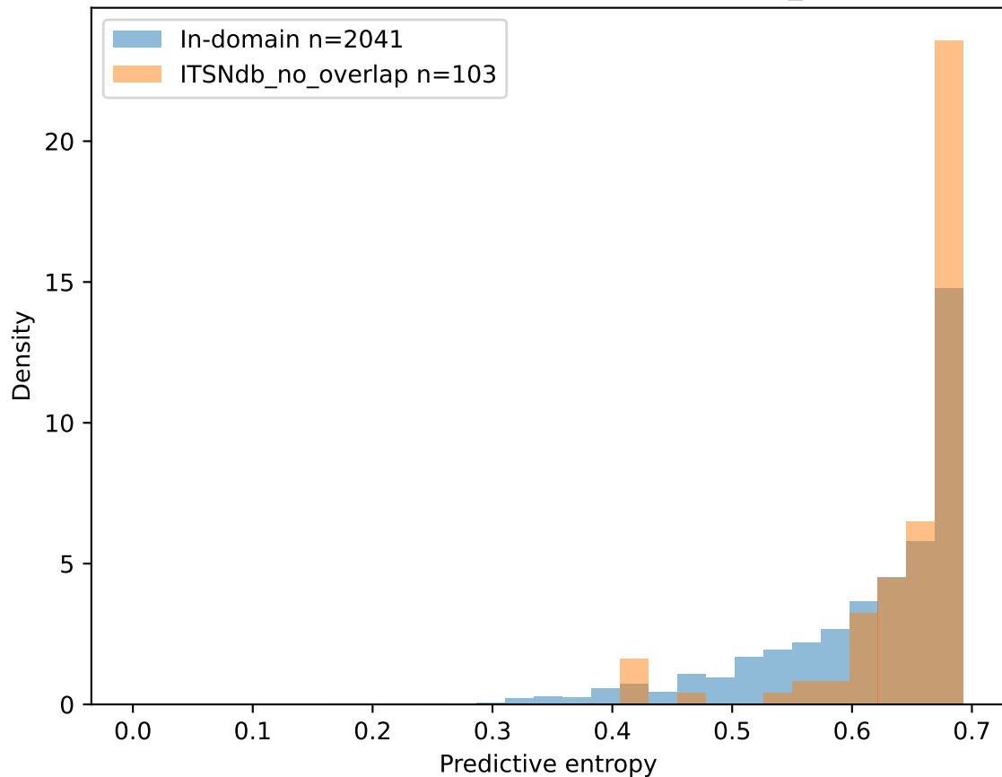
Uncertainty: in-domain vs OOD (ITSNdb no_overlap)
