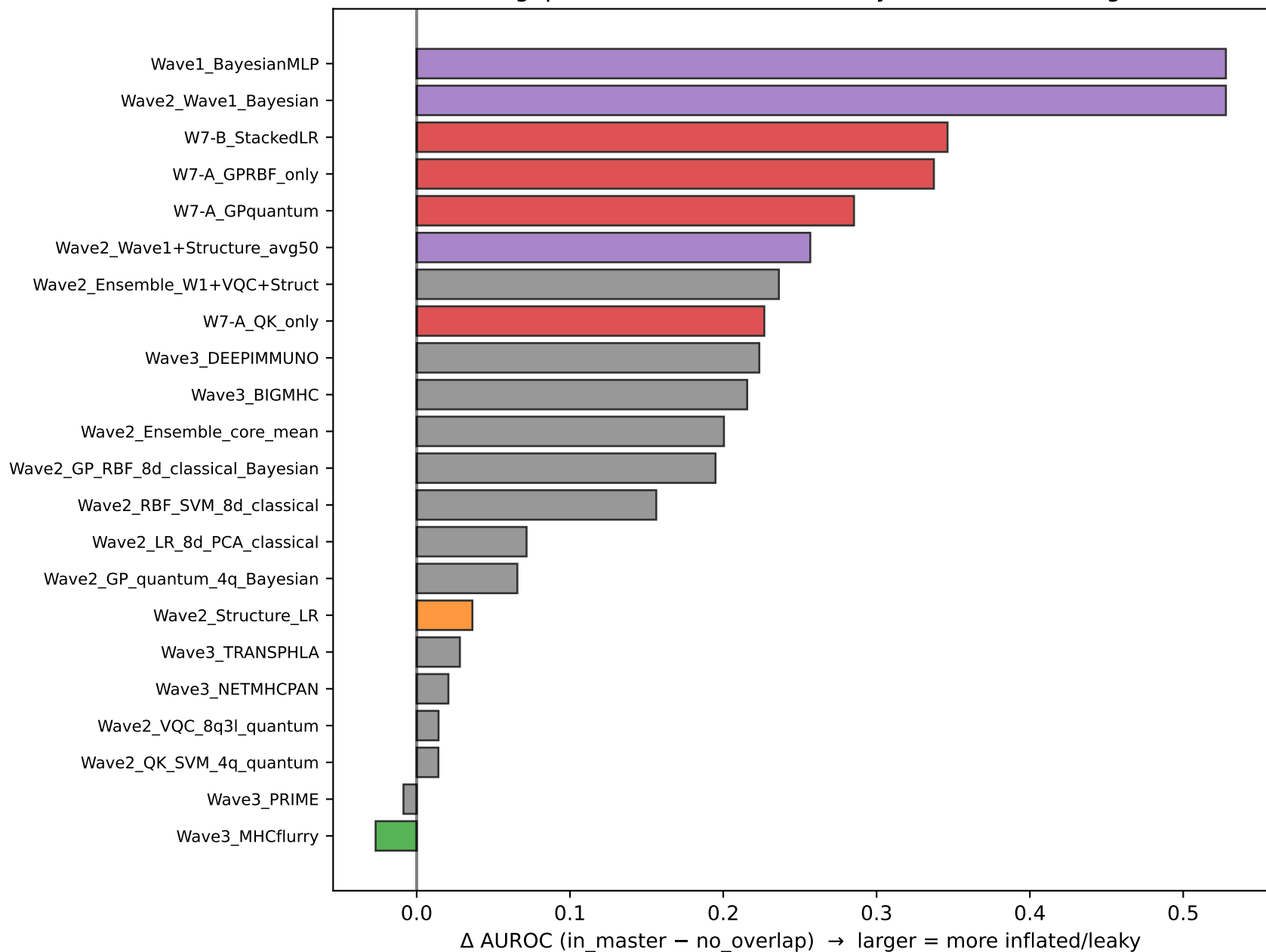
Wave 7 — Inflation gap across 17+ methods (truly held-out vs leakage-contaminated)
