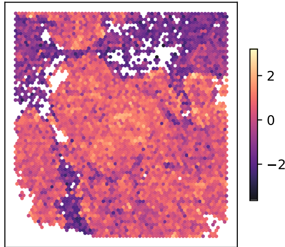
GSM7980867_PTC-4 JAK_8517 DPC-007448
