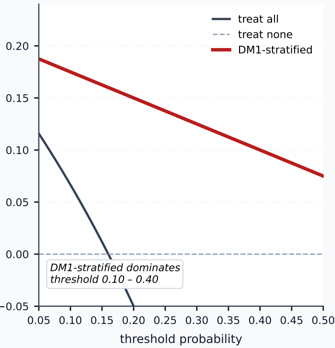
Decision-curve analysis
