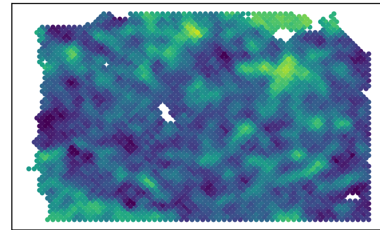
P4 observed
