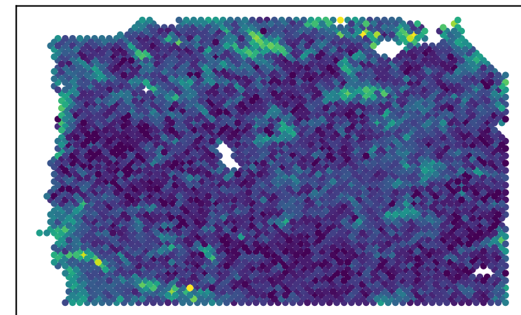
P4 H&E-predicted
