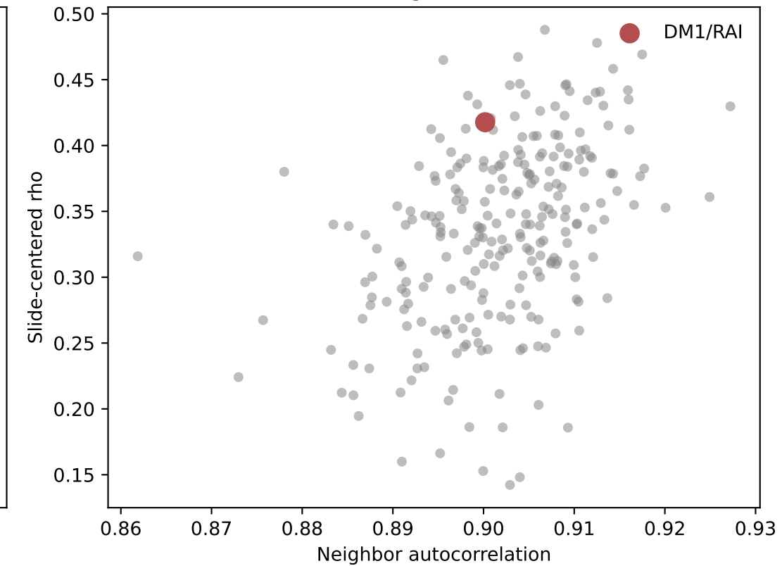
F. Residual rho vs neighbor autocorrelation
