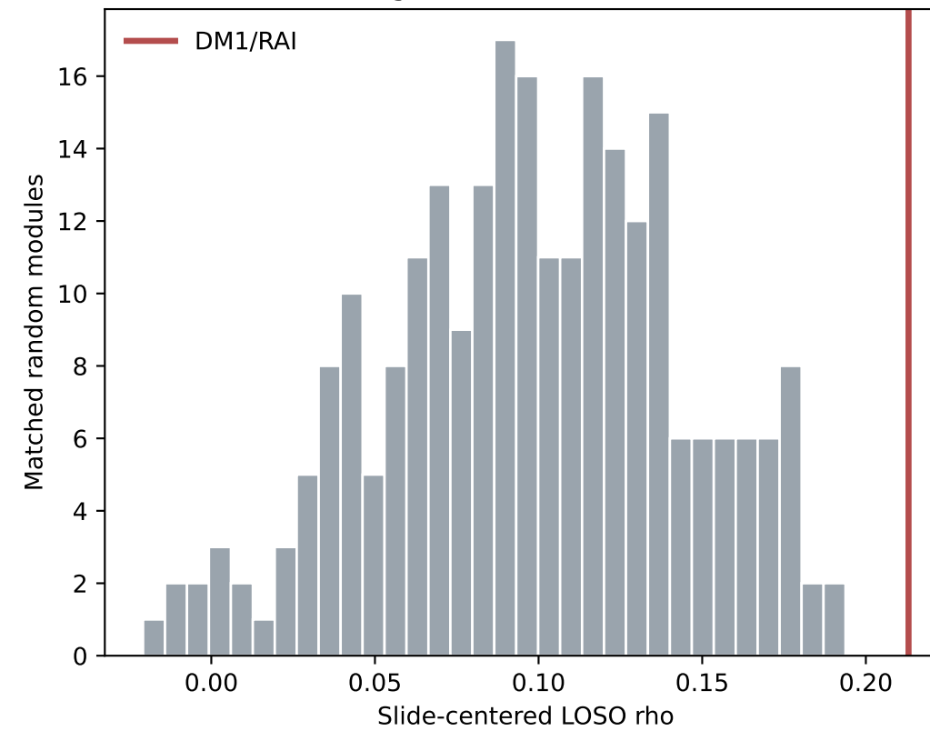
E. Residual-target smoothness-adjusted residual tail
