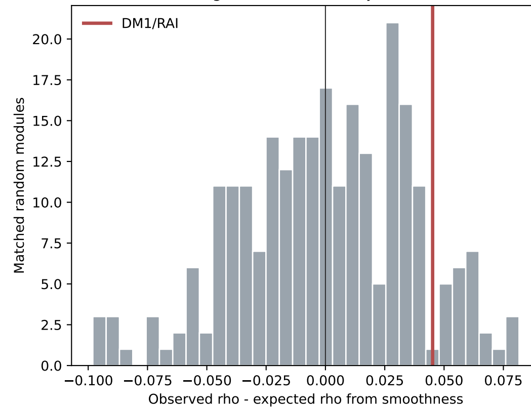
E. Residual-target smoothness-adjusted residual tail
