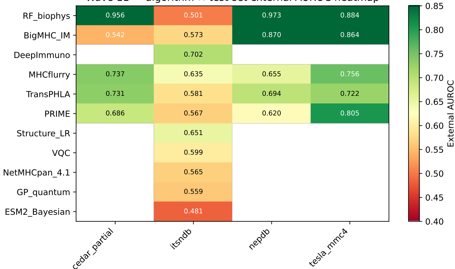
Wave 11 — algorithm × test-set external AUROC heatmap
