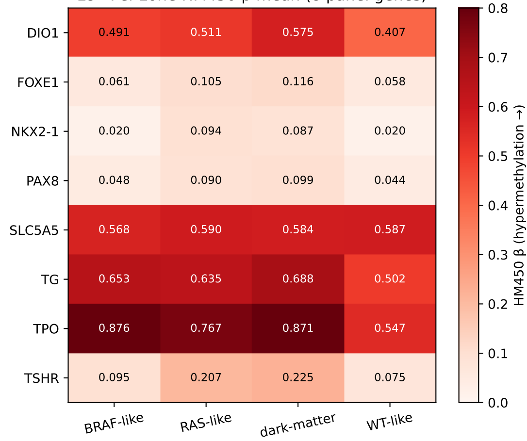
L8 · Per-zone HM450 \beta mean (8 panel genes)
