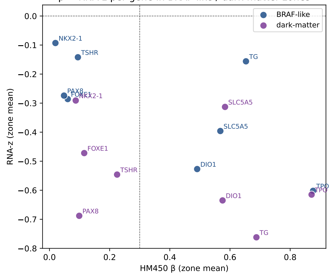
\beta \times RNA-z per gene in BRAF-like / dark-matter zones
