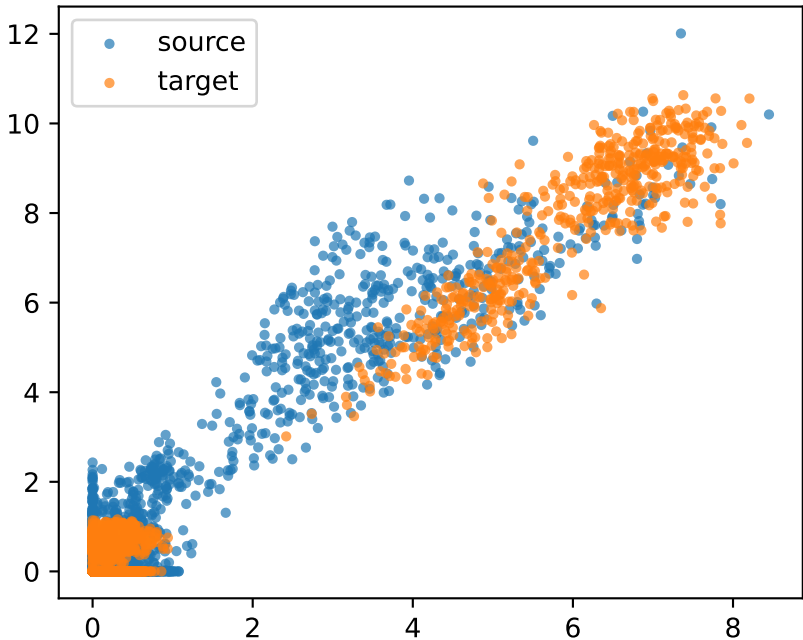
Domain embedding
