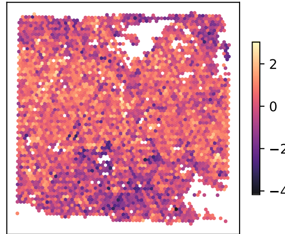
GSM7980869_LPTC-2 1E-1-(2-hydroxy-5-methylphenyl)-1-dodecanone-oxime
