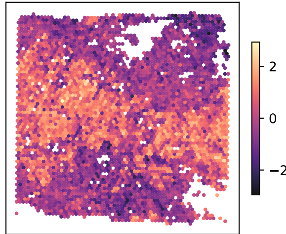
GSM7980869_LPTC-2 A12B4C3
